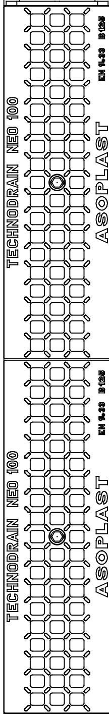
TCN100S BGS - NEO 100S + DUCTILE IRON GRATING B125
