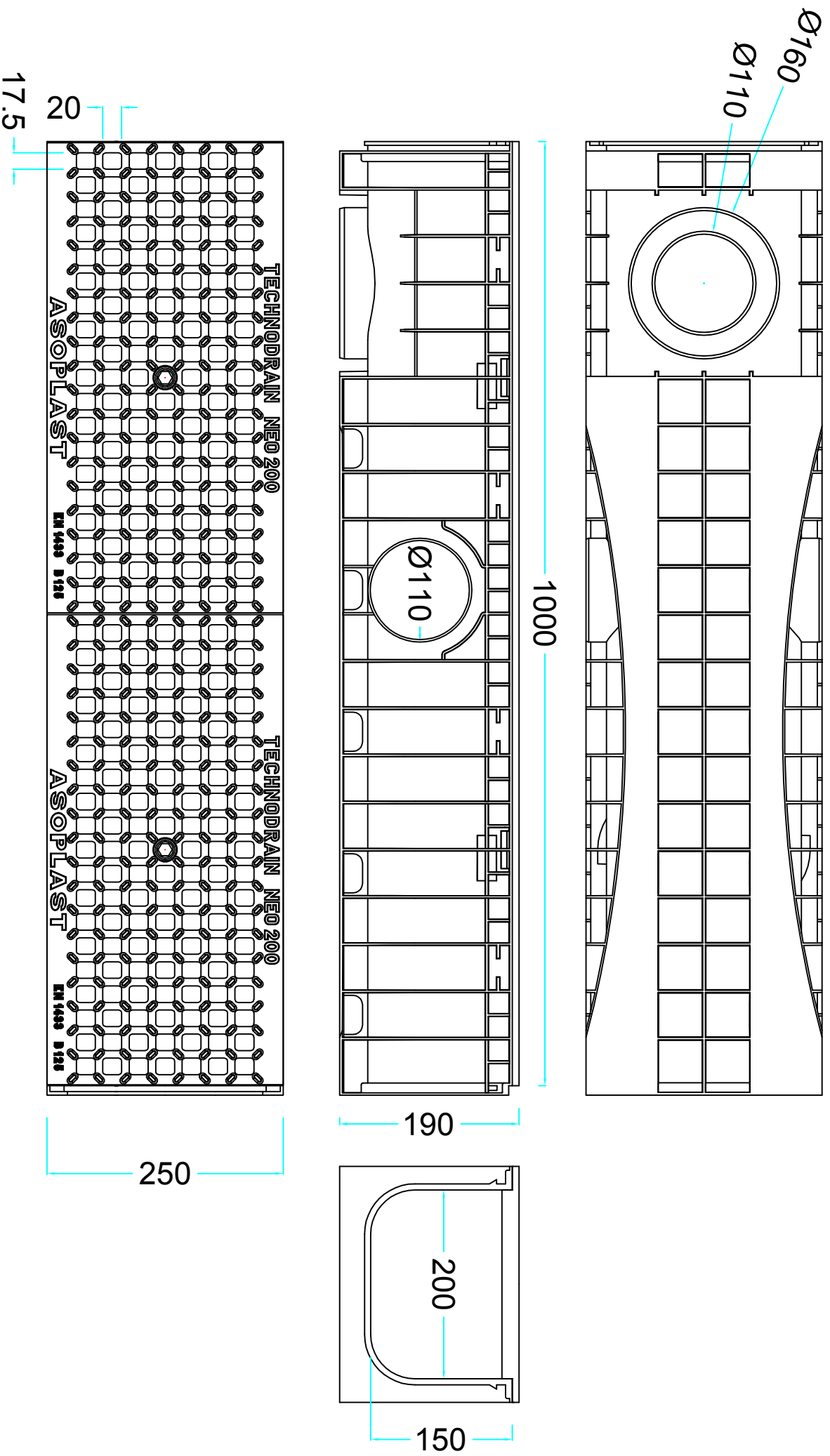
TCN200HBGS - NEO 200H + DUCTILE IRON GRATING B125
