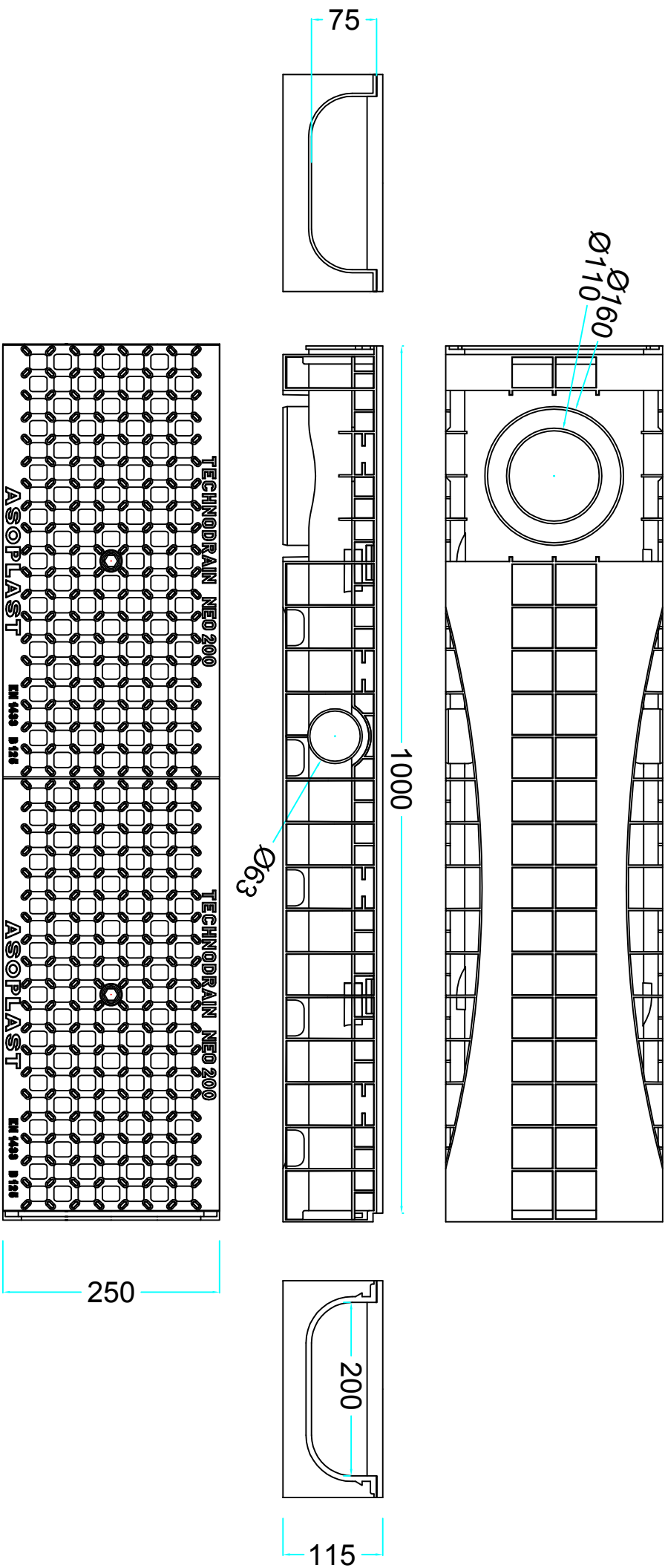
TCN200SBSGS - NEO 200S + DUCTILE IRON GRATING B125
