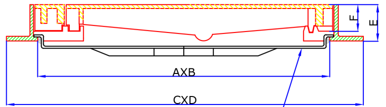
SECTIONAL VIEW
