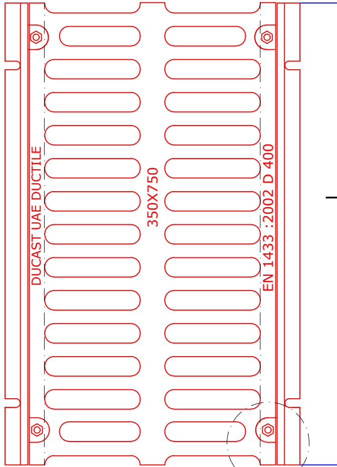
PLAN VIEW
